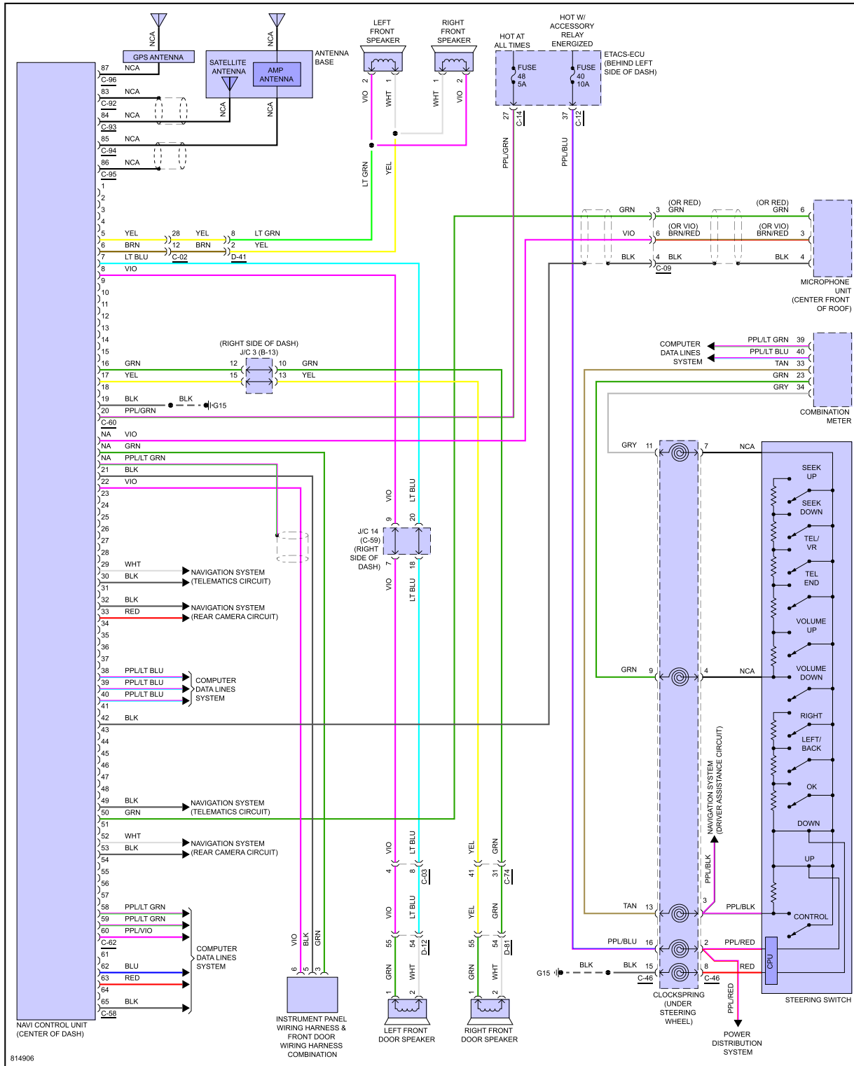
Fig 4: Radio Circuit, W/O Bose
