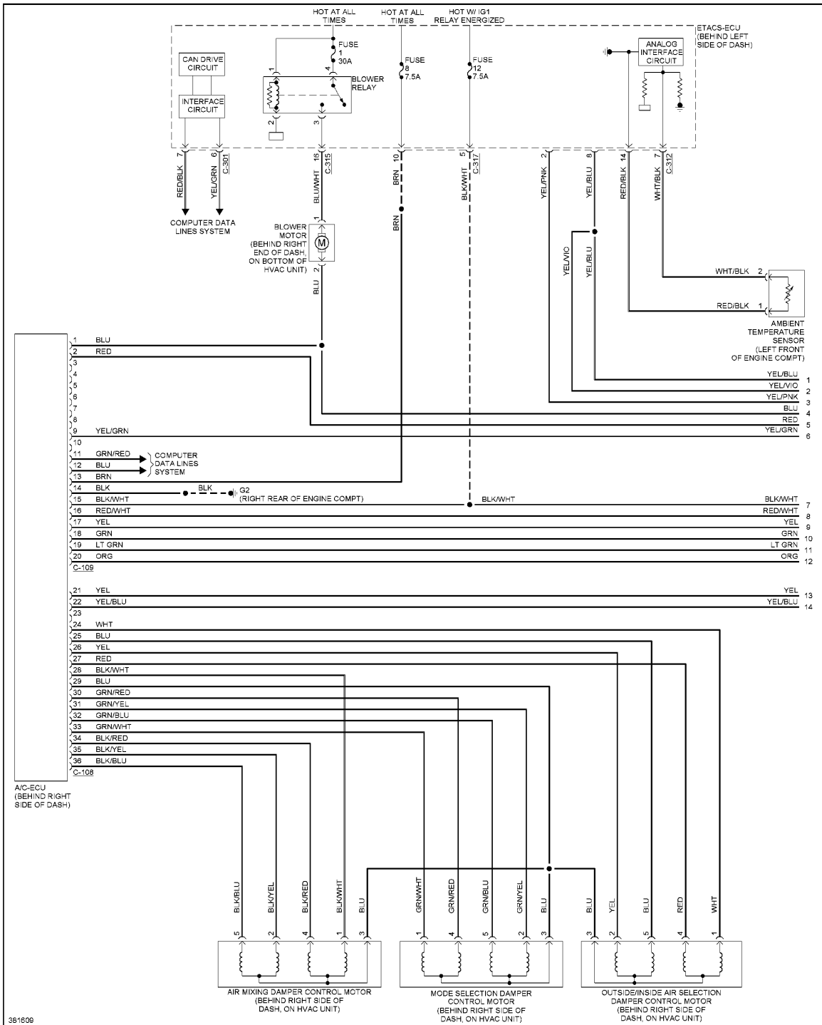
Fig. 1: 2.4L, Automatic A/C Circuit (1 of 3)
